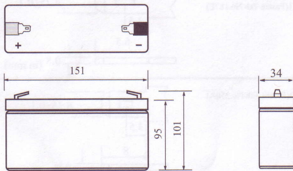
Dimensions (mm)
